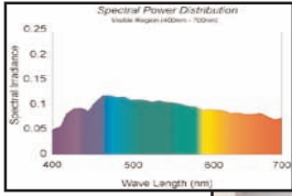
DAYLIGHT (CIE D65, 6500K) Full spectrum
