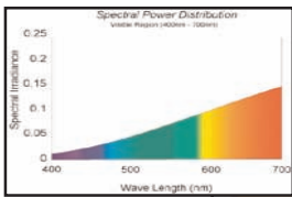
HOME LIGHT Incandescent (CIE 'A', 2856K)
