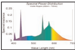
STORE LIGHT CWF (4100K) Green/yellow
